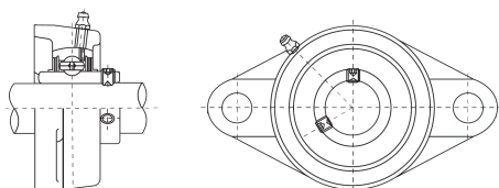
Supporto monoblcco in ghisa UCFL
