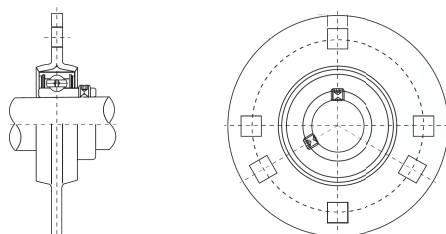
Supporto monoblcco in ghisa UCF
