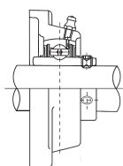
Supporto monoblcco in ghisa UCFL
